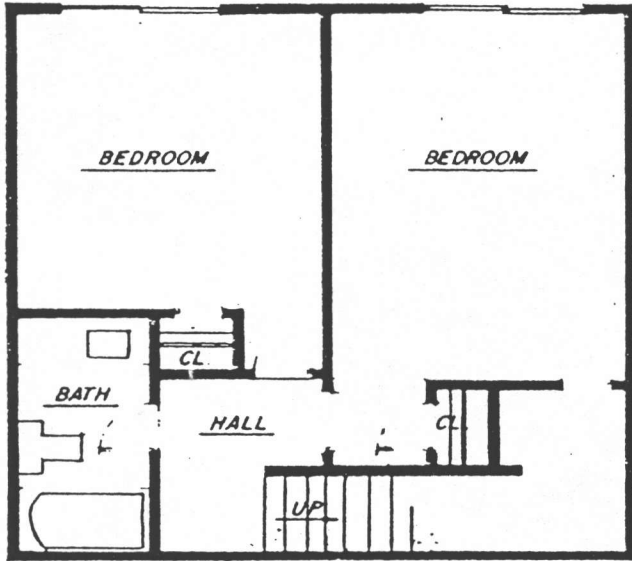
two bedroom "down" unit
